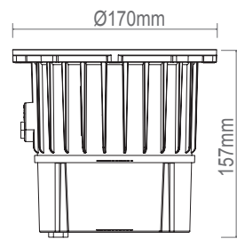
LED body
