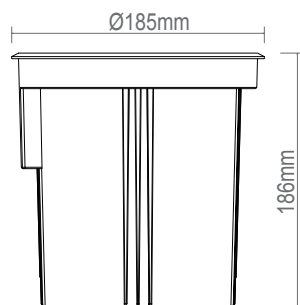
supplied housing
